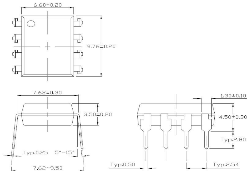
DIP8
